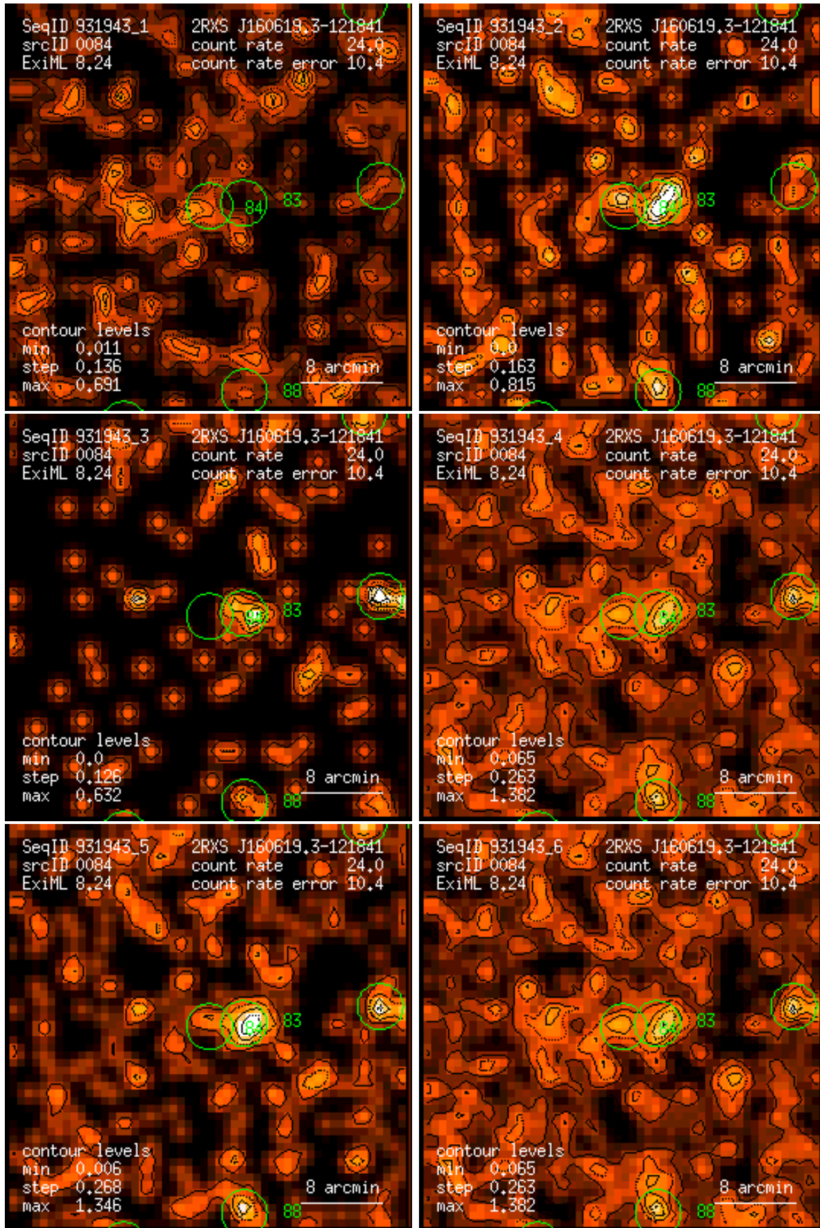
Figure 84: RASS 931943: detection 0084: band rate images, Gaussian filter: (1) PSPC channels 11 – 41, (2) 52 – 90, (3) 91 – 201, (4) 11 – 235, (5) 52 – 201, (6) 11 – 201. Broad band rates in counts/ks. Band rate contour levels in counts/ks/arcmin 2 .
