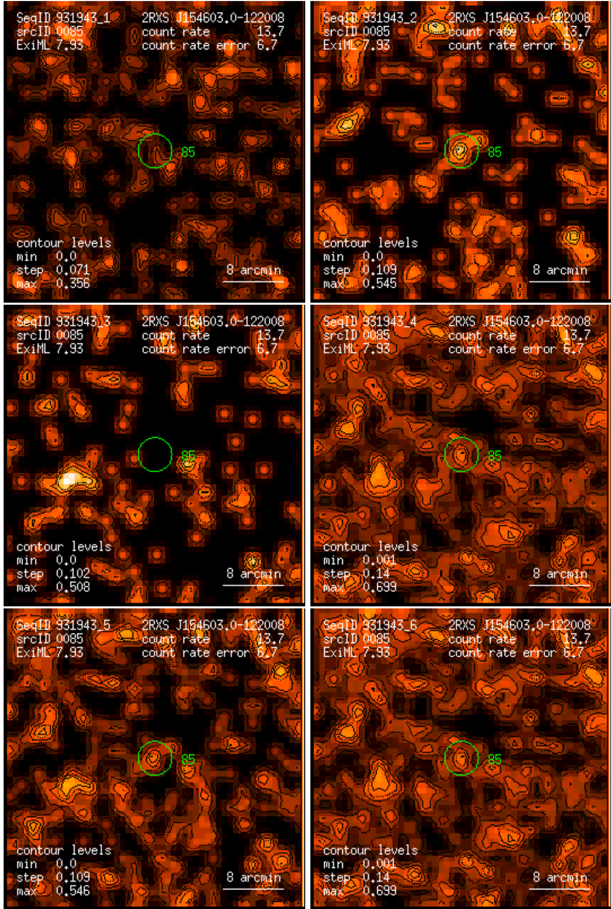
Figure 85: RASS 931943: detection 0085: band rate images, Gaussian filter: (1) PSPC channels 11 – 41, (2) 52 – 90, (3) 91 – 201, (4) 11 – 235, (5) 52 – 201, (6) 11 – 201. Broad band rates in counts/ks. Band rate contour levels in counts/ks/arcmin 2 .
