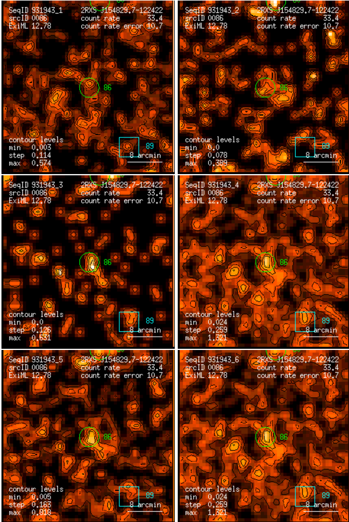
Figure 86: RASS 931943: detection 0086: band rate images, Gaussian filter: (1) PSPC channels 11 – 41, (2) 52 – 90, (3) 91 – 201, (4) 11 – 235, (5) 52 – 201, (6) 11 – 201. Broad band rates in counts/ks. Band rate contour levels in counts/ks/arcmin 2 .
