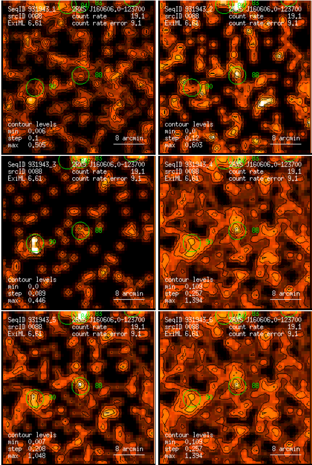
Figure 88: RASS 931943: detection 0088: band rate images, Gaussian filter: (1) PSPC channels 11 – 41, (2) 52 – 90, (3) 91 – 201, (4) 11 – 235, (5) 52 – 201, (6) 11 – 201. Broad band rates in counts/ks. Band rate contour levels in counts/ks/arcmin 2 .
