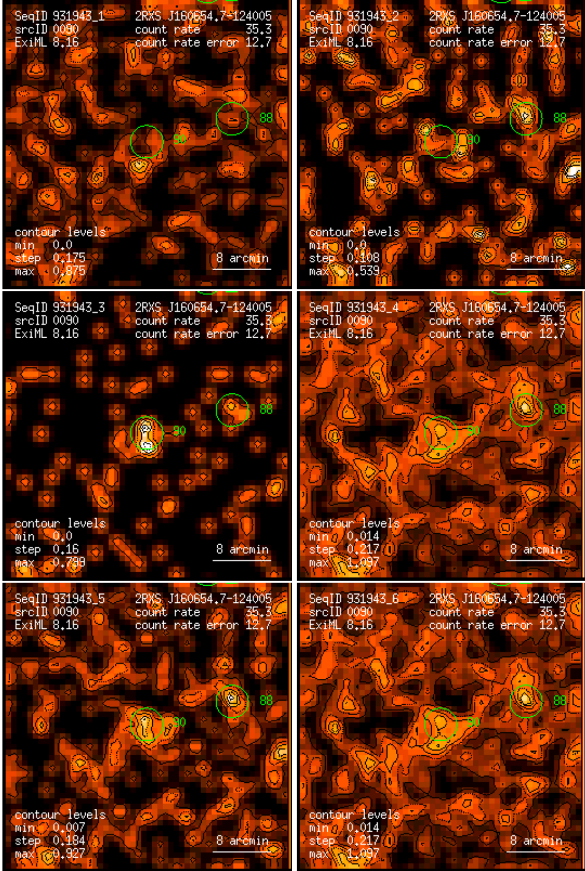
Figure 90: RASS 931943: detection 0090: band rate images, Gaussian filter: (1) PSPC channels 11 – 41, (2) 52 – 90, (3) 91 – 201, (4) 11 – 235, (5) 52 – 201, (6) 11 – 201. Broad band rates in counts/ks. Band rate contour levels in counts/ks/arcmin 2 .
