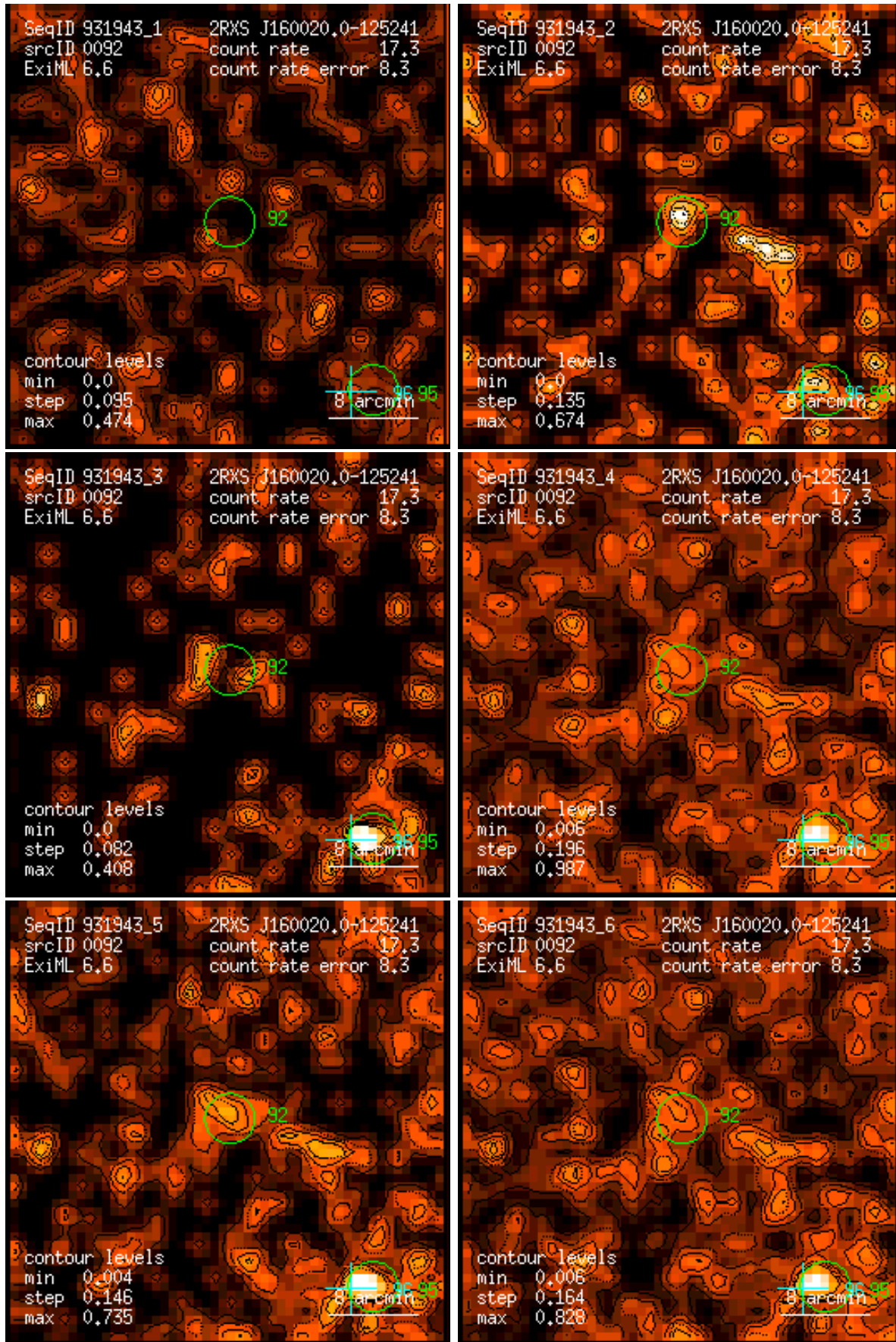
Figure 92: RASS 931943: detection 0092: band rate images, Gaussian filter: (1) PSPC channels 11 – 41, (2) 52 – 90, (3) 91 – 201, (4) 11 – 235, (5) 52 – 201, (6) 11 – 201. Broad band rates in counts/ks. Band rate contour levels in counts/ks/arcmin 2 .
