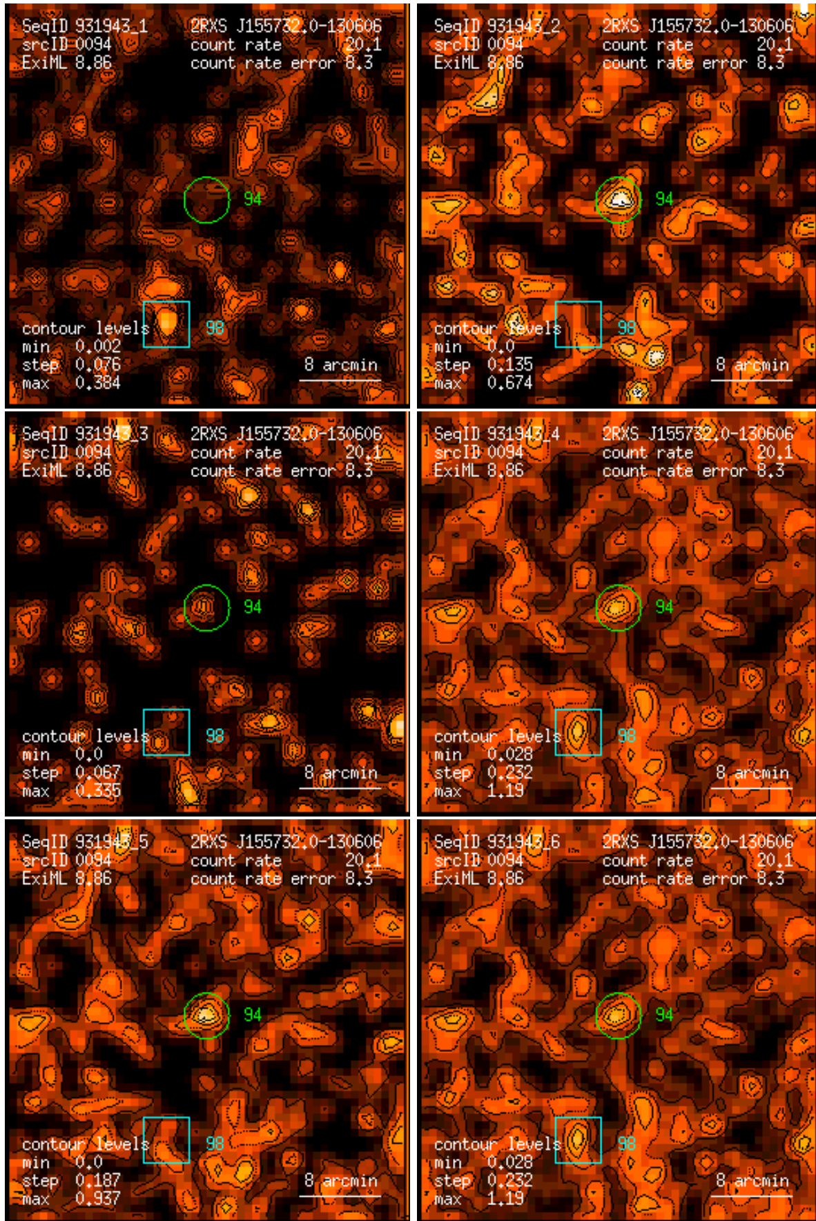
Figure 94: RASS 931943: detection 0094: band rate images, Gaussian filter: (1) PSPC channels 11 – 41, (2) 52 – 90, (3) 91 – 201, (4) 11 – 235, (5) 52 – 201, (6) 11 – 201. Broad band rates in counts/ks. Band rate contour levels in counts/ks/arcmin 2 .
