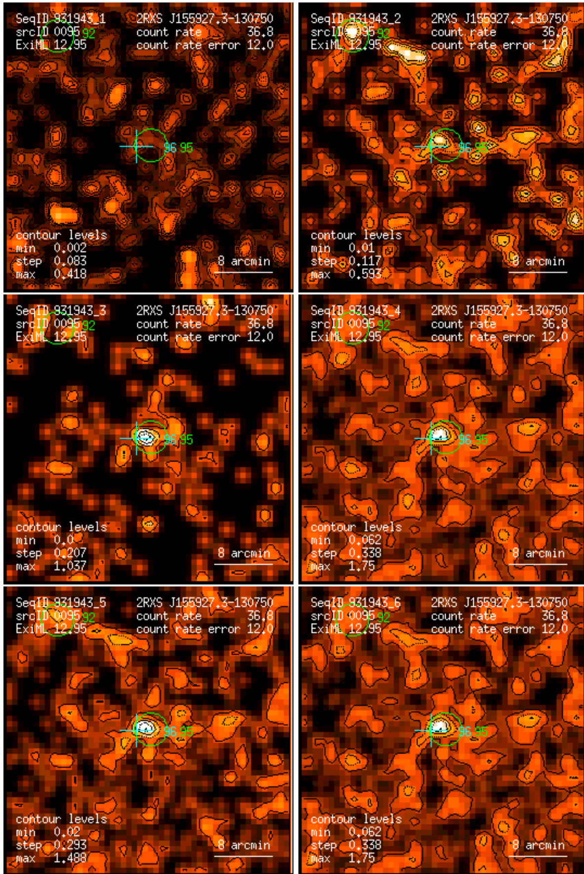
Figure 95: RASS 931943: detection 0095: band rate images, Gaussian filter: (1) PSPC channels 11 – 41, (2) 52 – 90, (3) 91 – 201, (4) 11 – 235, (5) 52 – 201, (6) 11 – 201. Broad band rates in counts/ks. Band rate contour levels in counts/ks/arcmin 2 .
