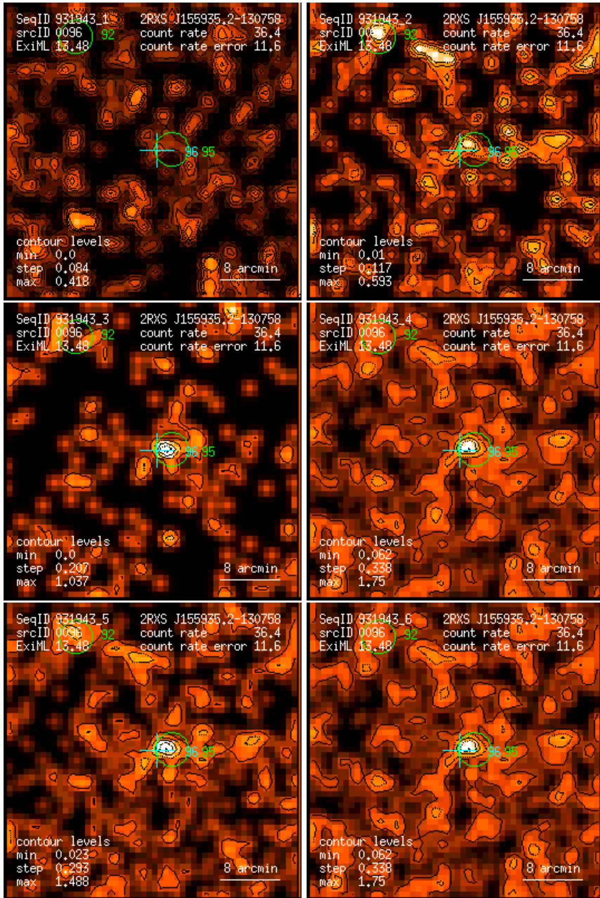
Figure 96: RASS 931943: detection 0096: band rate images, Gaussian filter: (1) PSPC channels 11 – 41, (2) 52 – 90, (3) 91 – 201, (4) 11 – 235, (5) 52 – 201, (6) 11 – 201. Broad band rates in counts/ks. Band rate contour levels in counts/ks/arcmin 2 .
