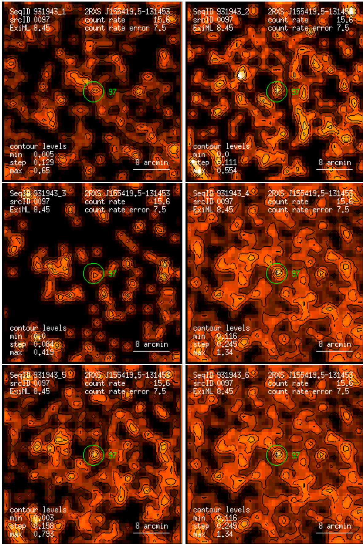
Figure 97: RASS 931943: detection 0097: band rate images, Gaussian filter: (1) PSPC channels 11 – 41, (2) 52 – 90, (3) 91 – 201, (4) 11 – 235, (5) 52 – 201, (6) 11 – 201. Broad band rates in counts/ks. Band rate contour levels in counts/ks/arcmin 2 .
