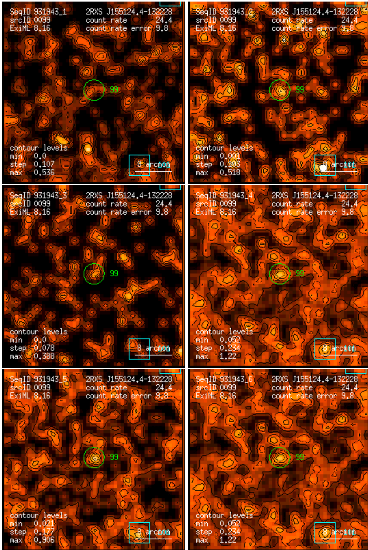
Figure 99: RASS 931943: detection 0099: band rate images, Gaussian filter: (1) PSPC channels 11 – 41, (2) 52 – 90, (3) 91 – 201, (4) 11 – 235, (5) 52 – 201, (6) 11 – 201. Broad band rates in counts/ks. Band rate contour levels in counts/ks/arcmin 2 .
