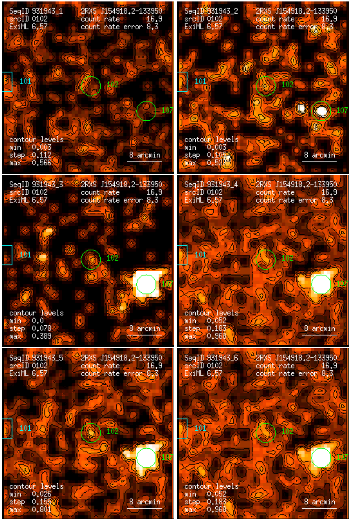
Figure 102: RASS 931943: detection 0102: band rate images, Gaussian filter: (1) PSPC channels 11 – 41, (2) 52 – 90, (3) 91 – 201, (4) 11 – 235, (5) 52 – 201, (6) 11 – 201. Broad band rates in counts/ks. Band rate contour levels in counts/ks/arcmin 2 .
