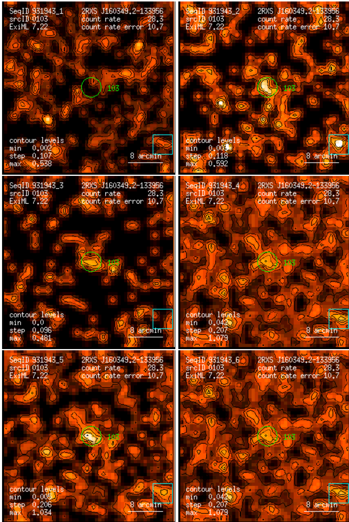
Figure 103: RASS 931943: detection 0103: band rate images, Gaussian filter: (1) PSPC channels 11 – 41, (2) 52 – 90, (3) 91 – 201, (4) 11 – 235, (5) 52 – 201, (6) 11 – 201. Broad band rates in counts/ks. Band rate contour levels in counts/ks/arcmin 2 .
