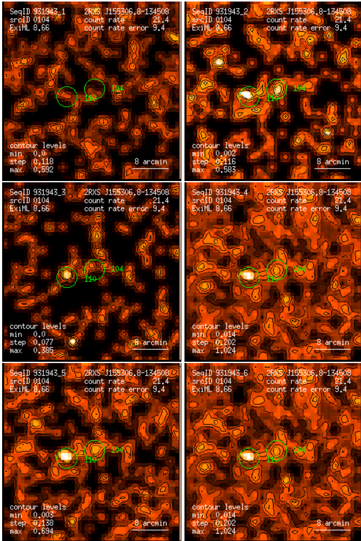
Figure 104: RASS 931943: detection 0104: band rate images, Gaussian filter: (1) PSPC channels 11 – 41, (2) 52 – 90, (3) 91 – 201, (4) 11 – 235, (5) 52 – 201, (6) 11 – 201. Broad band rates in counts/ks. Band rate contour levels in counts/ks/arcmin 2 .
