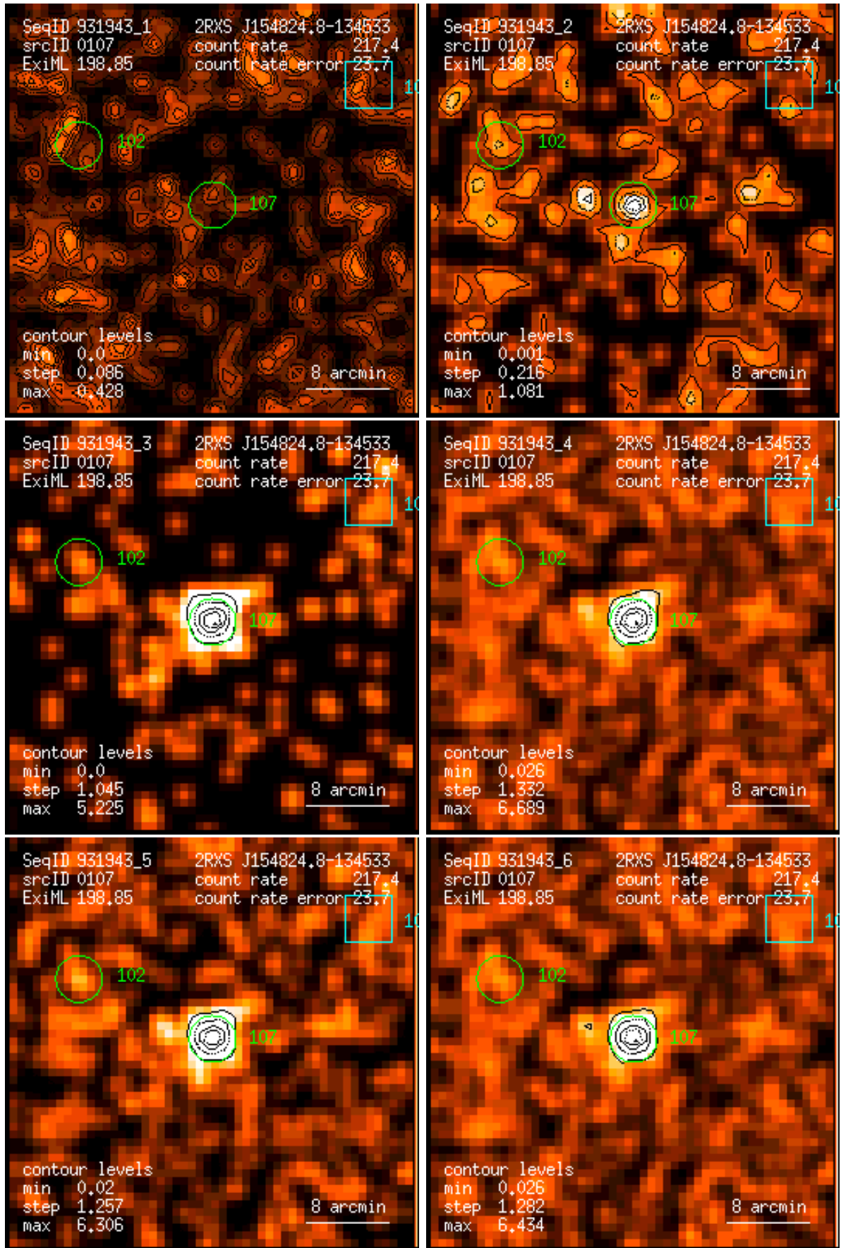
Figure 107: RASS 931943: detection 0107: band rate images, Gaussian filter: (1) PSPC channels 11 – 41, (2) 52 – 90, (3) 91 – 201, (4) 11 – 235, (5) 52 – 201, (6) 11 – 201. Broad band rates in counts/ks. Band rate contour levels in counts/ks/arcmin 2 .
