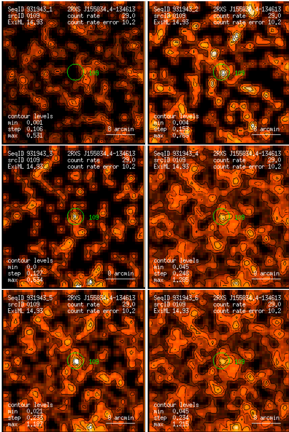
Figure 109: RASS 931943: detection 0109: band rate images, Gaussian filter: (1) PSPC channels 11 – 41, (2) 52 – 90, (3) 91 – 201, (4) 11 – 235, (5) 52 – 201, (6) 11 – 201. Broad band rates in counts/ks. Band rate contour levels in counts/ks/arcmin 2 .
