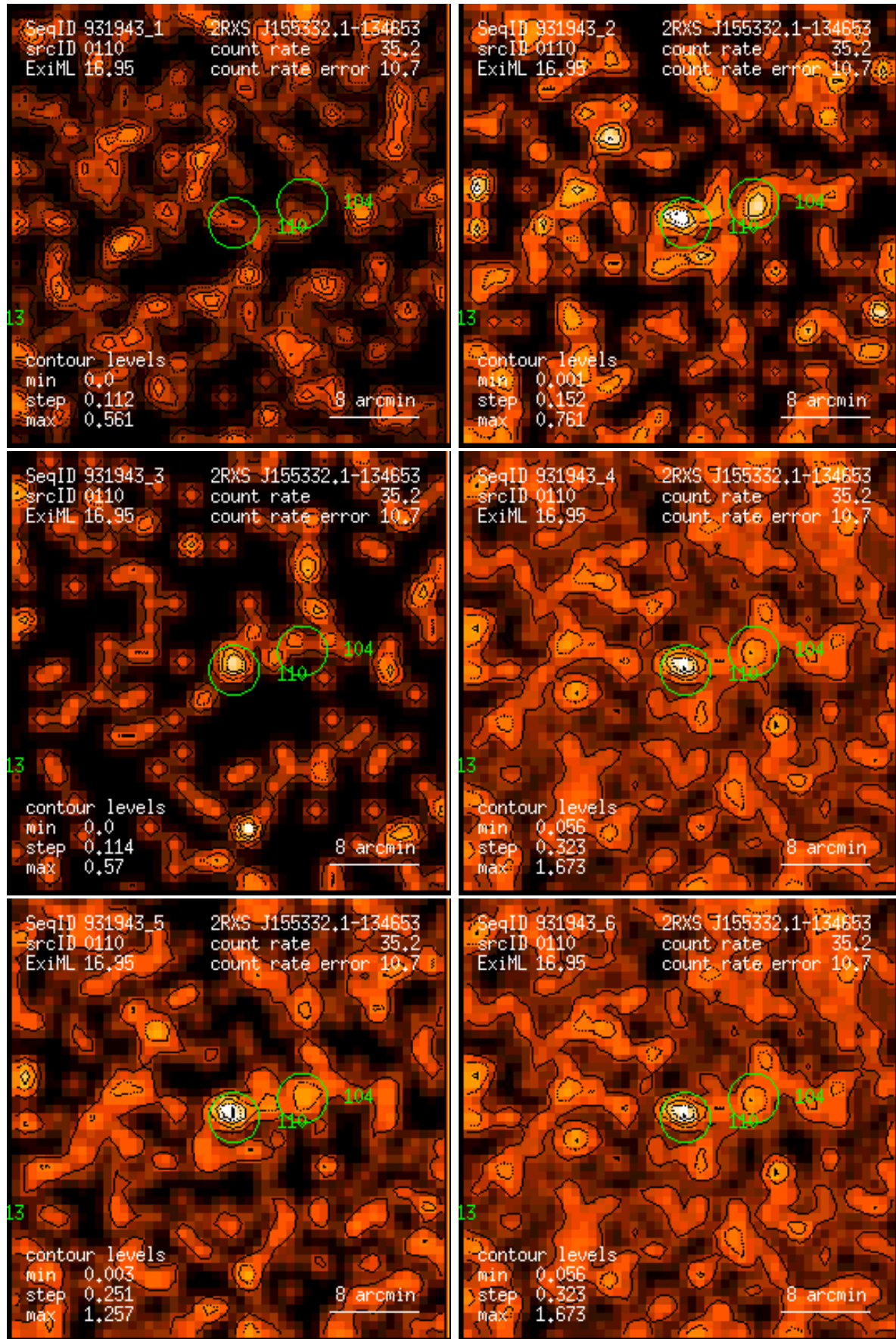
Figure 110: RASS 931943: detection 0110: band rate images, Gaussian filter: (1) PSPC channels 11 – 41, (2) 52 – 90, (3) 91 – 201, (4) 11 – 235, (5) 52 – 201, (6) 11 – 201. Broad band rates in counts/ks. Band rate contour levels in counts/ks/arcmin 2 .
