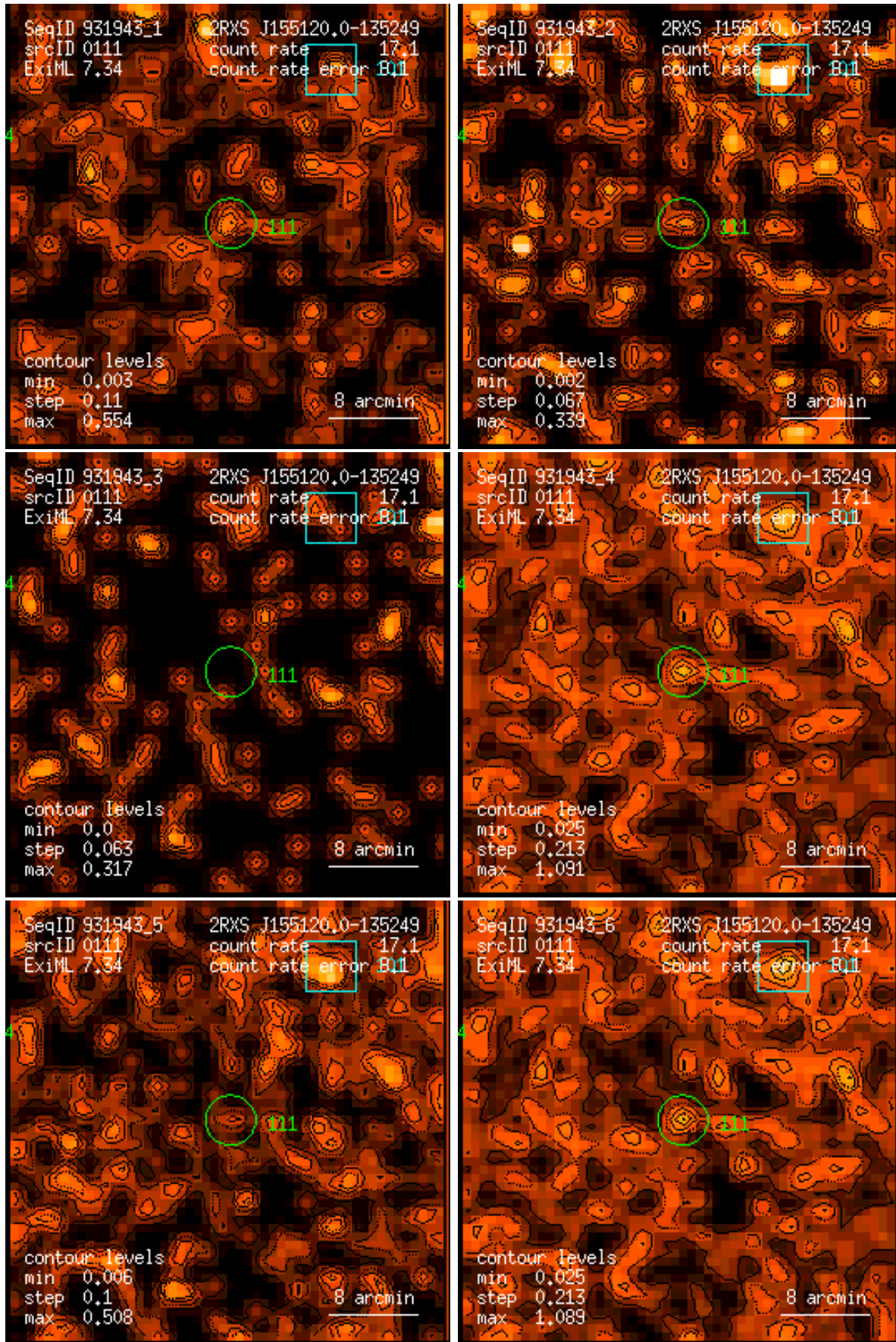
Figure 111: RASS 931943: detection 0111: band rate images, Gaussian filter: (1) PSPC channels 11 – 41, (2) 52 – 90, (3) 91 – 201, (4) 11 – 235, (5) 52 – 201, (6) 11 – 201. Broad band rates in counts/ks. Band rate contour levels in counts/ks/arcmin 2 .
