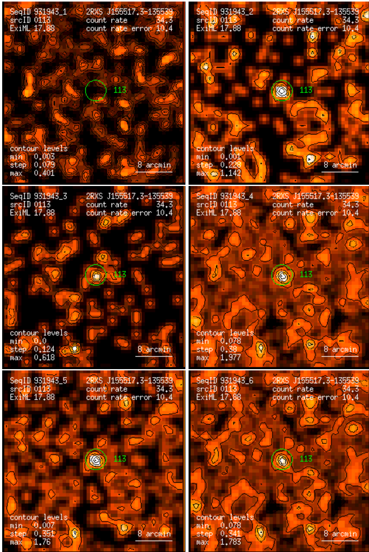
Figure 113: RASS 931943: detection 0113: band rate images, Gaussian filter: (1) PSPC channels 11 – 41, (2) 52 – 90, (3) 91 – 201, (4) 11 – 235, (5) 52 – 201, (6) 11 – 201. Broad band rates in counts/ks. Band rate contour levels in counts/ks/arcmin 2 .
