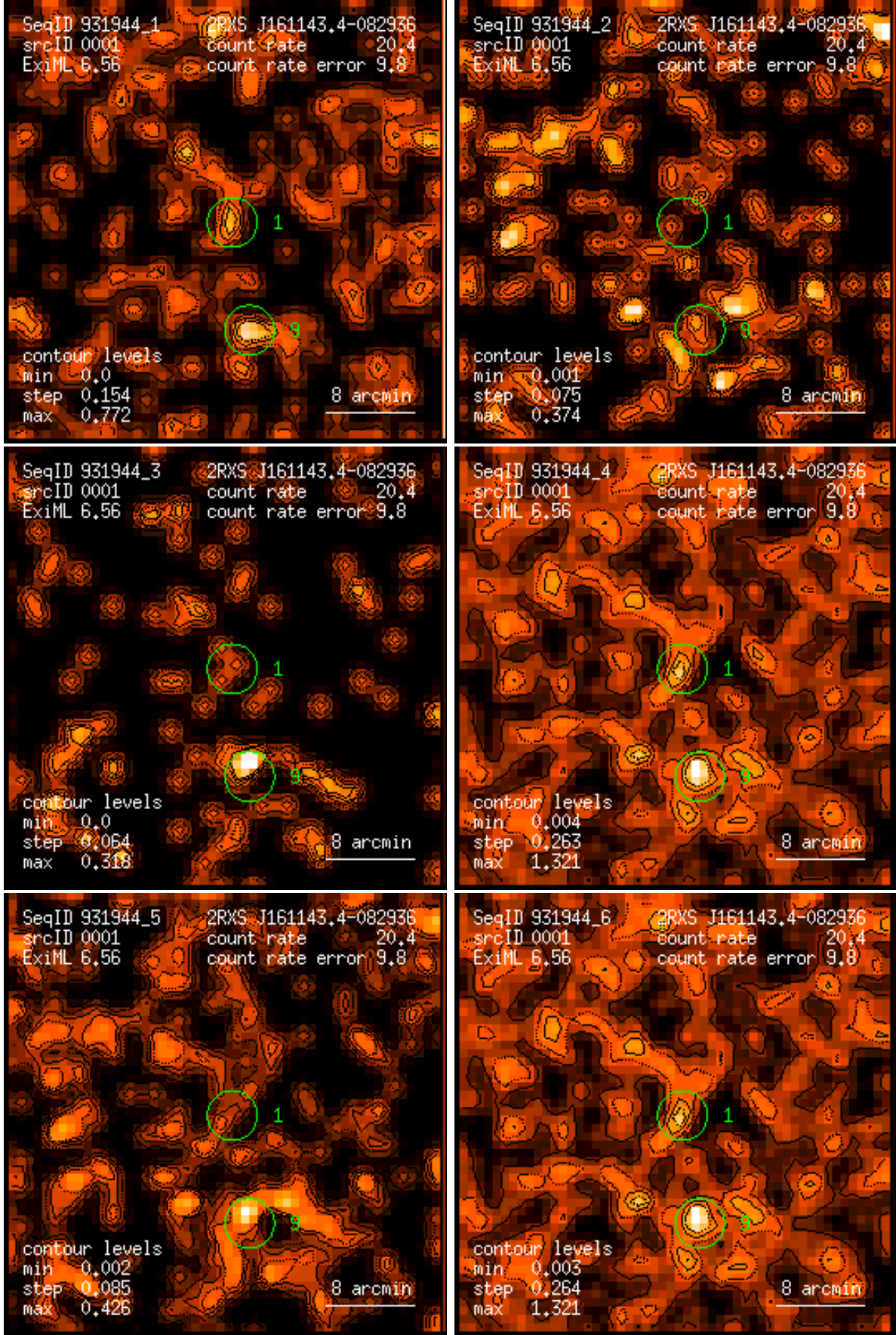
Figure 1: RASS 931944: detection 0001: band rate images, Gaussian filter: (1) PSPC channels 11 – 41, (2) 52 – 90, (3) 91 – 201, (4) 11 – 235, (5) 52 – 201, (6) 11 – 201. Broad band rates in counts/ks. Band rate contour levels in counts/ks/arcmin 2 .
