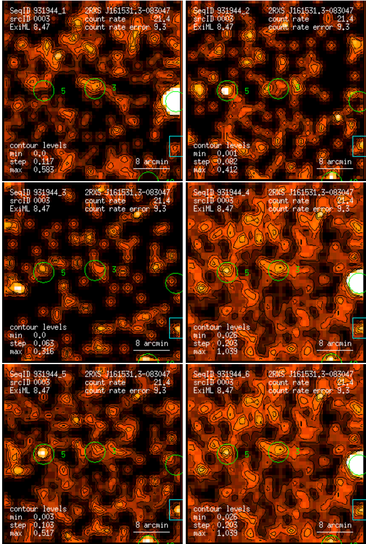
Figure 3: RASS 931944: detection 0003: band rate images, Gaussian filter: (1) PSPC channels 11 – 41, (2) 52 – 90, (3) 91 – 201, (4) 11 – 235, (5) 52 – 201, (6) 11 – 201. Broad band rates in counts/ks. Band rate contour levels in counts/ks/arcmin 2 .
