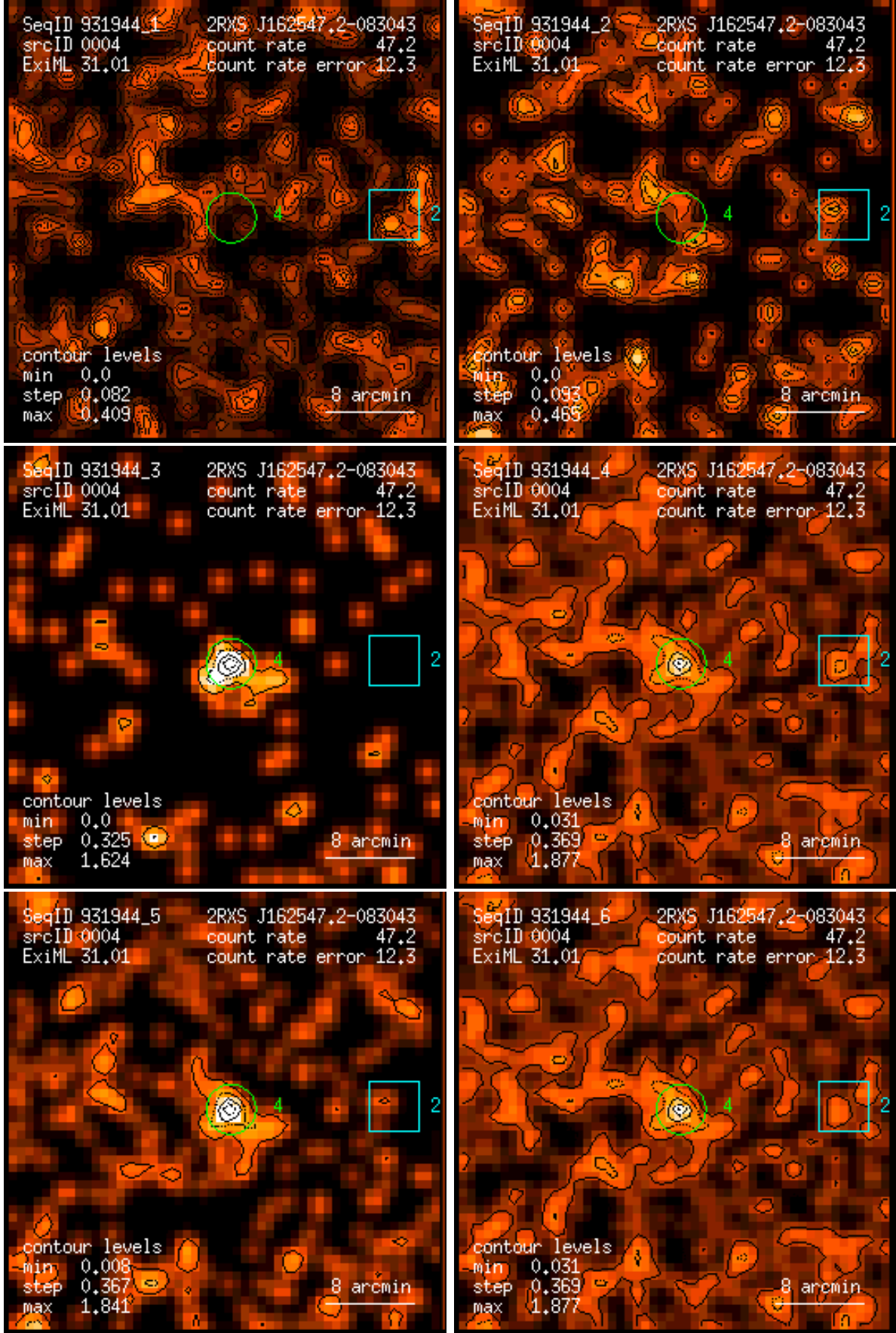
Figure 4: RASS 931944: detection 0004: band rate images, Gaussian filter: (1) PSPC channels 11 – 41, (2) 52 – 90, (3) 91 – 201, (4) 11 – 235, (5) 52 – 201, (6) 11 – 201. Broad band rates in counts/ks. Band rate contour levels in counts/ks/arcmin 2 .
