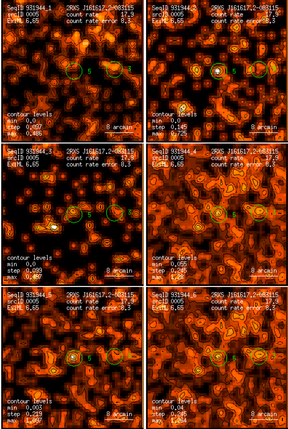
Figure 5: RASS 931944: detection 0005: band rate images, Gaussian filter: (1) PSPC channels 11 – 41, (2) 52 – 90, (3) 91 – 201, (4) 11 – 235, (5) 52 – 201, (6) 11 – 201. Broad band rates in counts/ks. Band rate contour levels in counts/ks/arcmin 2 .
