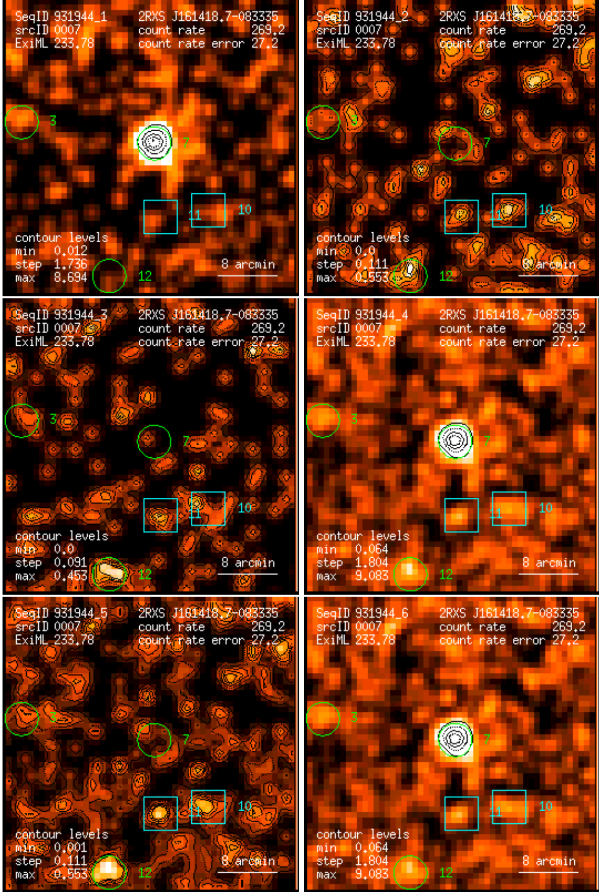
Figure 7: RASS 931944: detection 0007: band rate images, Gaussian filter: (1) PSPC channels 11 – 41, (2) 52 – 90, (3) 91 – 201, (4) 11 – 235, (5) 52 – 201, (6) 11 – 201. Broad band rates in counts/ks. Band rate contour levels in counts/ks/arcmin 2 .
