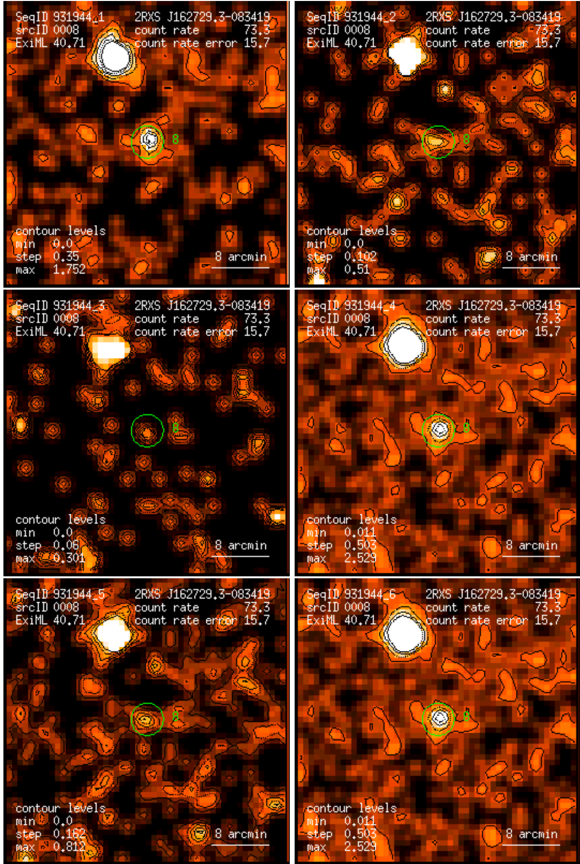
Figure 8: RASS 931944: detection 0008: band rate images, Gaussian filter: (1) PSPC channels 11 – 41, (2) 52 – 90, (3) 91 – 201, (4) 11 – 235, (5) 52 – 201, (6) 11 – 201. Broad band rates in counts/ks. Band rate contour levels in counts/ks/arcmin 2 .
