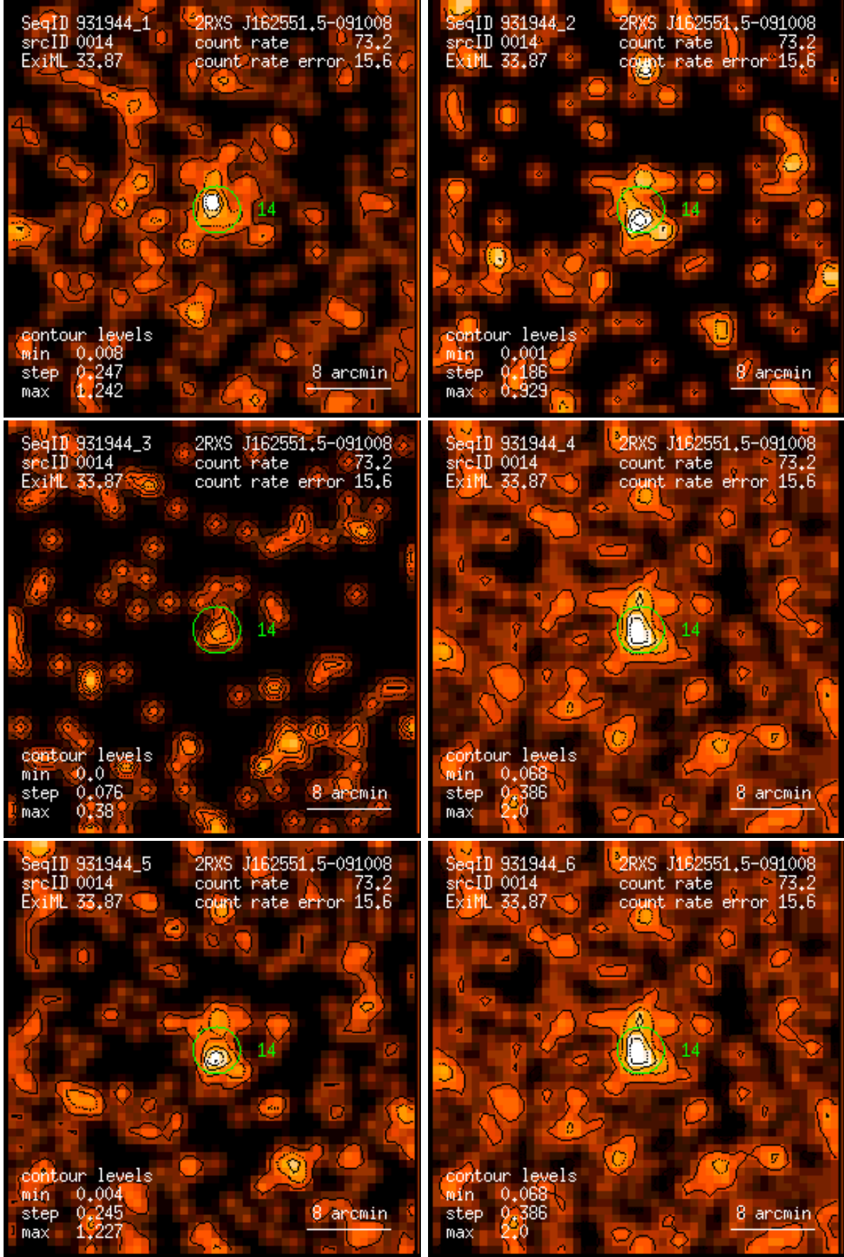
Figure 14: RASS 931944: detection 0014: band rate images, Gaussian filter: (1) PSPC channels 11 – 41, (2) 52 – 90, (3) 91 – 201, (4) 11 – 235, (5) 52 – 201, (6) 11 – 201. Broad band rates in counts/ks. Band rate contour levels in counts/ks/arcmin 2 .
