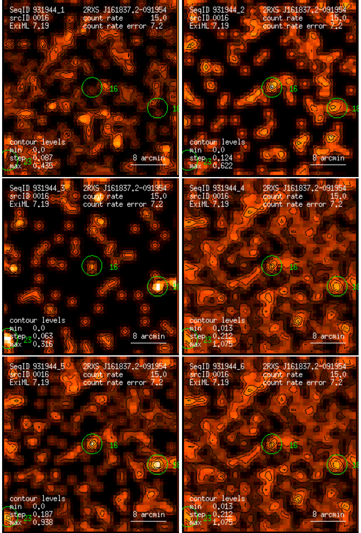
Figure 16: RASS 931944: detection 0016: band rate images, Gaussian filter: (1) PSPC channels 11 – 41, (2) 52 – 90, (3) 91 – 201, (4) 11 – 235, (5) 52 – 201, (6) 11 – 201. Broad band rates in counts/ks. Band rate contour levels in counts/ks/arcmin 2 .
