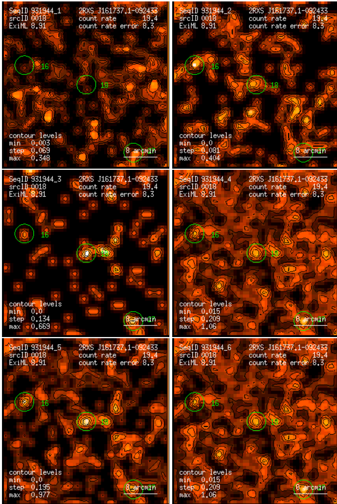
Figure 18: RASS 931944: detection 0018: band rate images, Gaussian filter: (1) PSPC channels 11 – 41, (2) 52 – 90, (3) 91 – 201, (4) 11 – 235, (5) 52 – 201, (6) 11 – 201. Broad band rates in counts/ks. Band rate contour levels in counts/ks/arcmin 2 .
