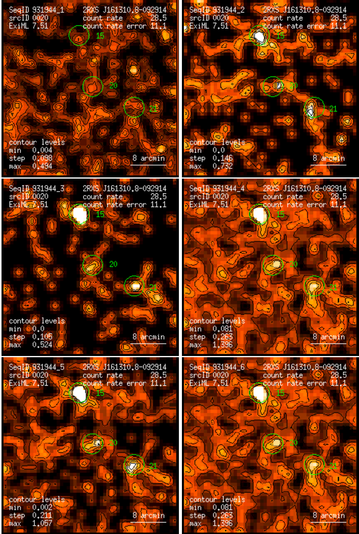
Figure 20: RASS 931944: detection 0020: band rate images, Gaussian filter: (1) PSPC channels 11 – 41, (2) 52 – 90, (3) 91 – 201, (4) 11 – 235, (5) 52 – 201, (6) 11 – 201. Broad band rates in counts/ks. Band rate contour levels in counts/ks/arcmin 2 .
