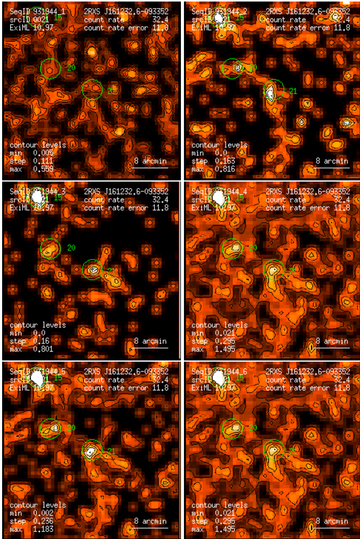
Figure 21: RASS 931944: detection 0021: band rate images, Gaussian filter: (1) PSPC channels 11 – 41, (2) 52 – 90, (3) 91 – 201, (4) 11 – 235, (5) 52 – 201, (6) 11 – 201. Broad band rates in counts/ks. Band rate contour levels in counts/ks/arcmin 2 .
