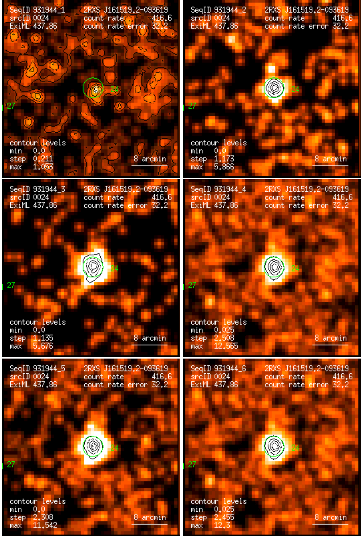
Figure 24: RASS 931944: detection 0024: band rate images, Gaussian filter: (1) PSPC channels 11 – 41, (2) 52 – 90, (3) 91 – 201, (4) 11 – 235, (5) 52 – 201, (6) 11 – 201. Broad band rates in counts/ks. Band rate contour levels in counts/ks/arcmin 2 .
