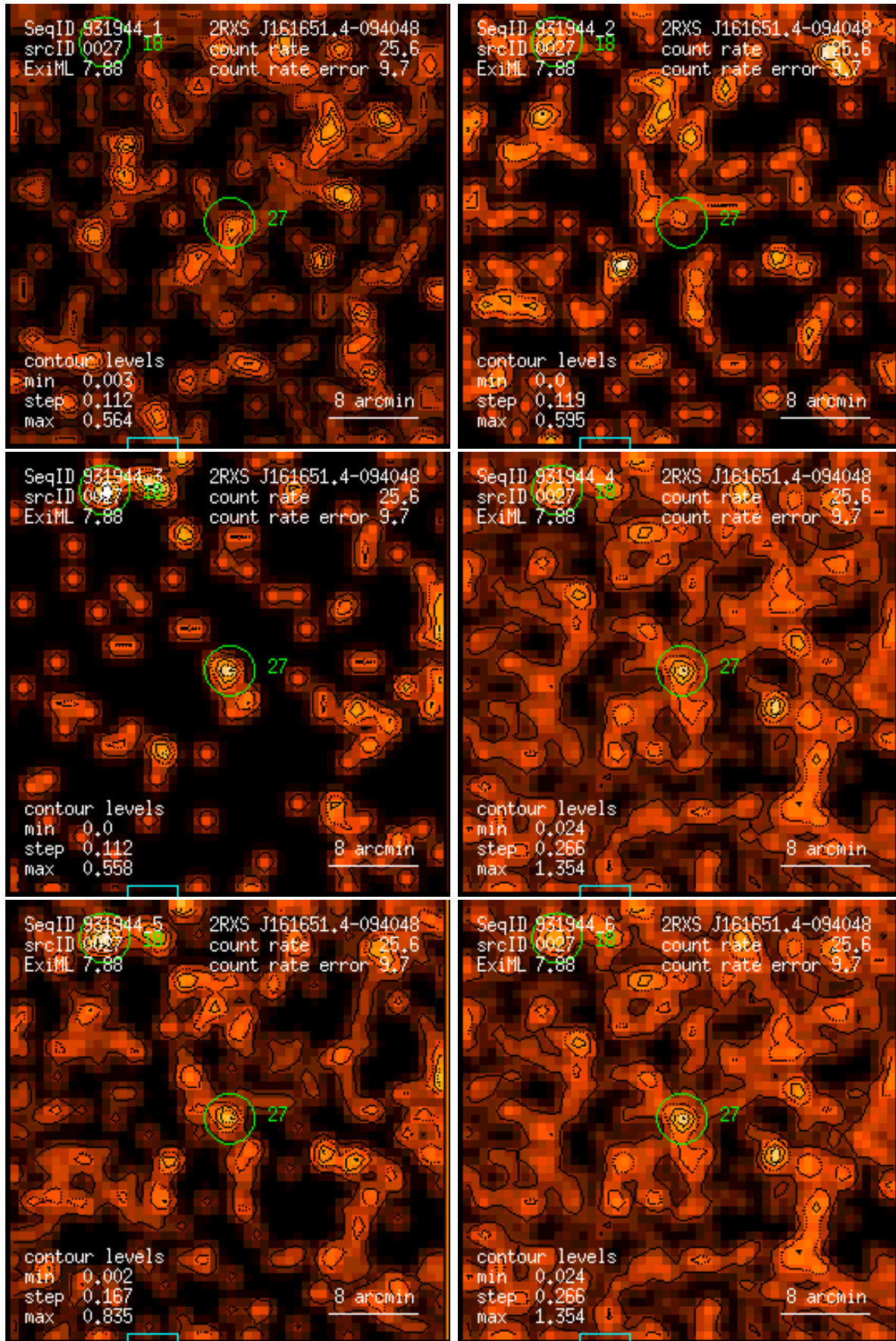
Figure 27: RASS 931944: detection 0027: band rate images, Gaussian filter: (1) PSPC channels 11 – 41, (2) 52 – 90, (3) 91 – 201, (4) 11 – 235, (5) 52 – 201, (6) 11 – 201. Broad band rates in counts/ks. Band rate contour levels in counts/ks/arcmin 2 .
