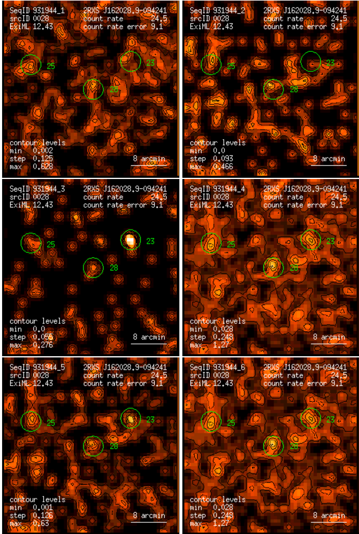
Figure 28: RASS 931944: detection 0028: band rate images, Gaussian filter: (1) PSPC channels 11 – 41, (2) 52 – 90, (3) 91 – 201, (4) 11 – 235, (5) 52 – 201, (6) 11 – 201. Broad band rates in counts/ks. Band rate contour levels in counts/ks/arcmin 2 .
