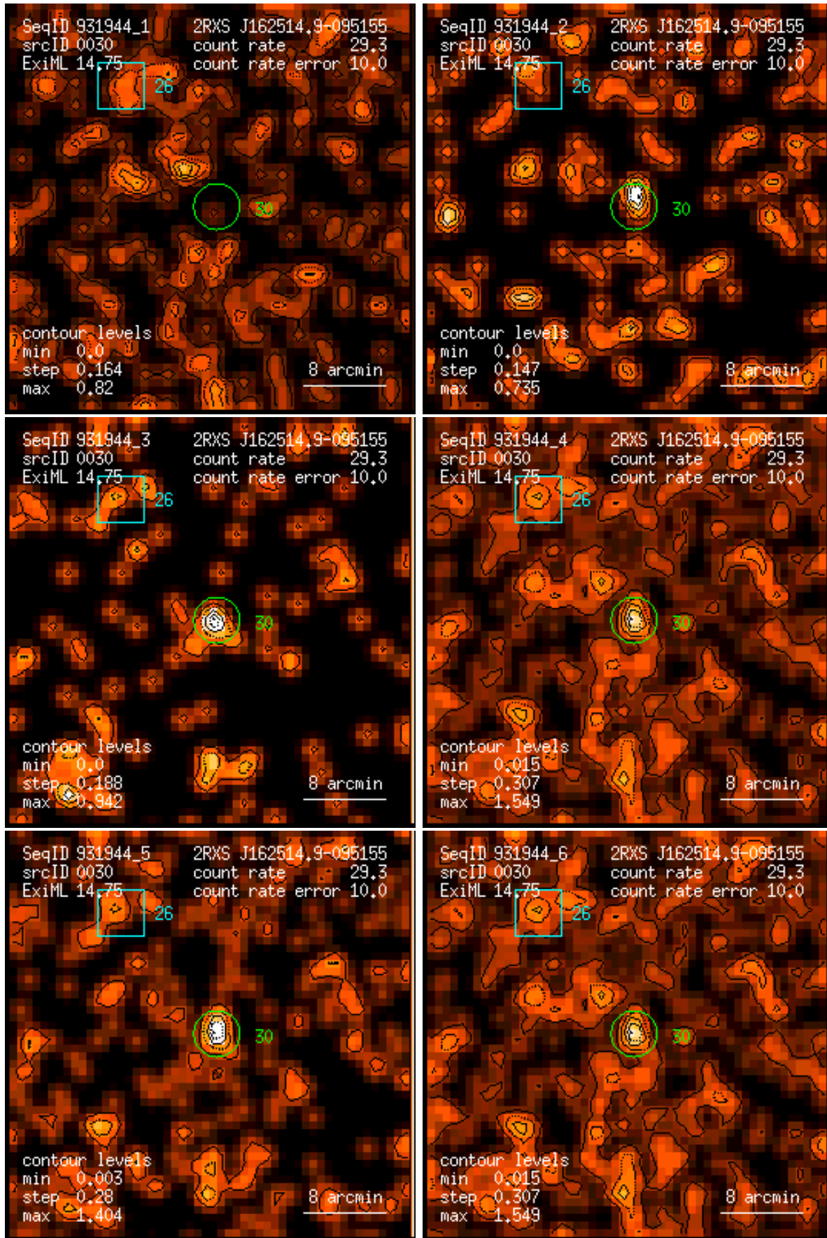
Figure 30: RASS 931944: detection 0030: band rate images, Gaussian filter: (1) PSPC channels 11 – 41, (2) 52 – 90, (3) 91 – 201, (4) 11 – 235, (5) 52 – 201, (6) 11 – 201. Broad band rates in counts/ks. Band rate contour levels in counts/ks/arcmin 2 .
