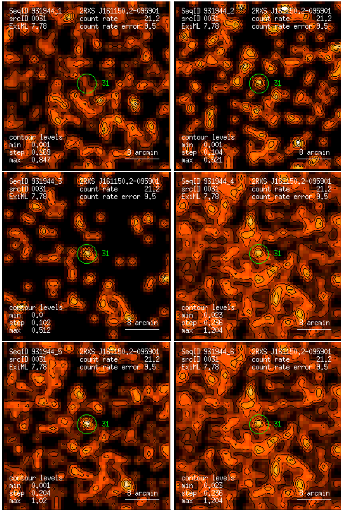
Figure 31: RASS 931944: detection 0031: band rate images, Gaussian filter: (1) PSPC channels 11 – 41, (2) 52 – 90, (3) 91 – 201, (4) 11 – 235, (5) 52 – 201, (6) 11 – 201. Broad band rates in counts/ks. Band rate contour levels in counts/ks/arcmin 2 .
