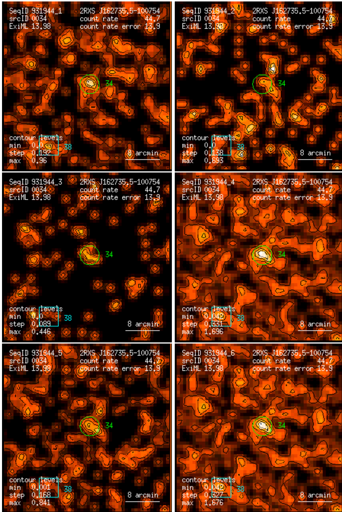
Figure 34: RASS 931944: detection 0034: band rate images, Gaussian filter: (1) PSPC channels 11 – 41, (2) 52 – 90, (3) 91 – 201, (4) 11 – 235, (5) 52 – 201, (6) 11 – 201. Broad band rates in counts/ks. Band rate contour levels in counts/ks/arcmin 2 .
