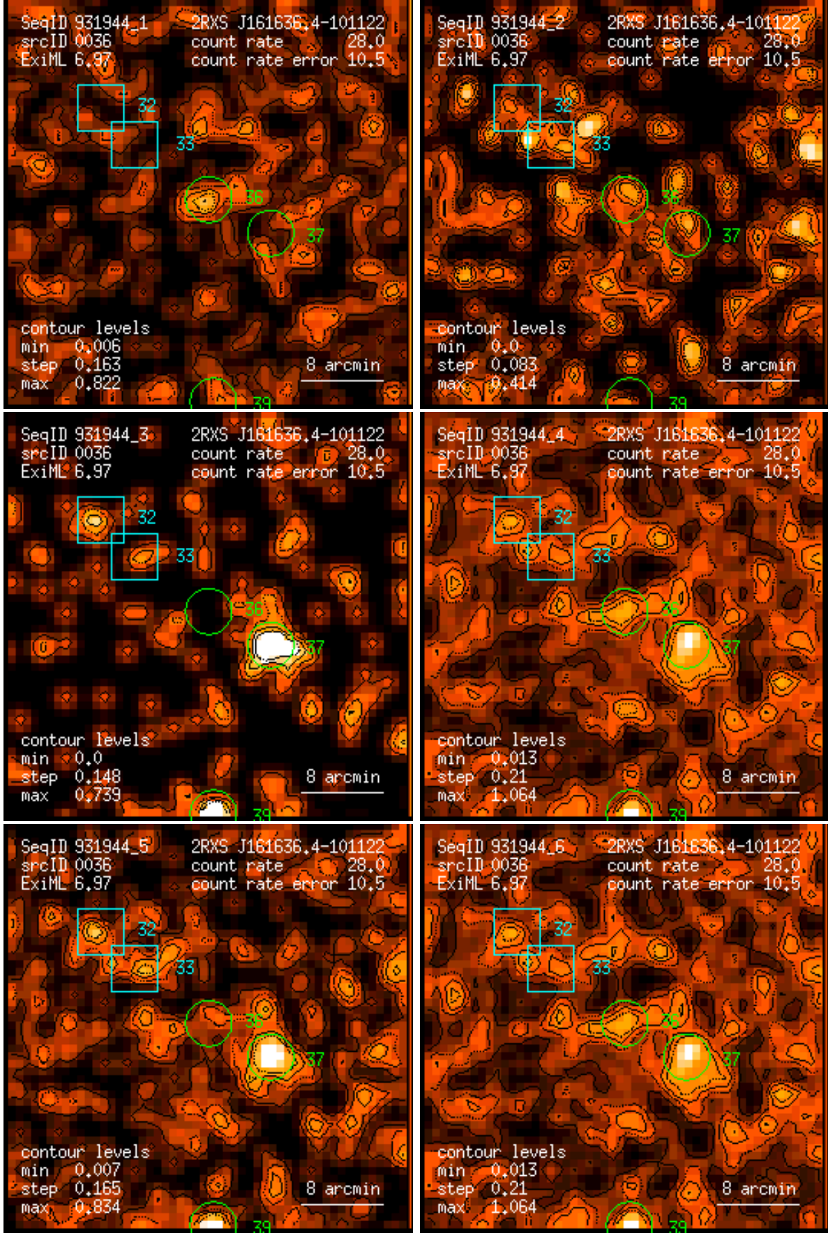
Figure 36: RASS 931944: detection 0036: band rate images, Gaussian filter: (1) PSPC channels 11 – 41, (2) 52 – 90, (3) 91 – 201, (4) 11 – 235, (5) 52 – 201, (6) 11 – 201. Broad band rates in counts/ks. Band rate contour levels in counts/ks/arcmin 2 .
