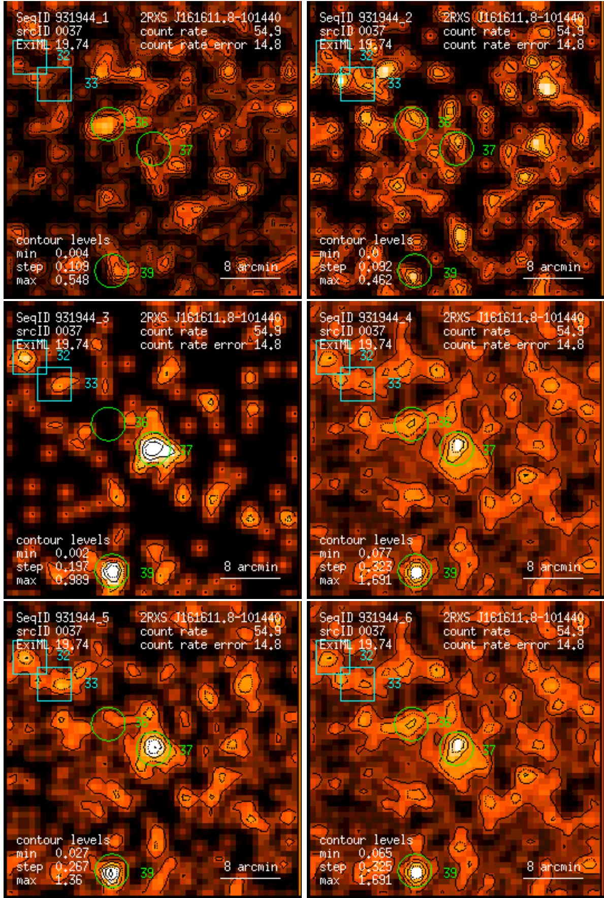
Figure 37: RASS 931944: detection 0037: band rate images, Gaussian filter: (1) PSPC channels 11 – 41, (2) 52 – 90, (3) 91 – 201, (4) 11 – 235, (5) 52 – 201, (6) 11 – 201. Broad band rates in counts/ks. Band rate contour levels in counts/ks/arcmin 2 .
