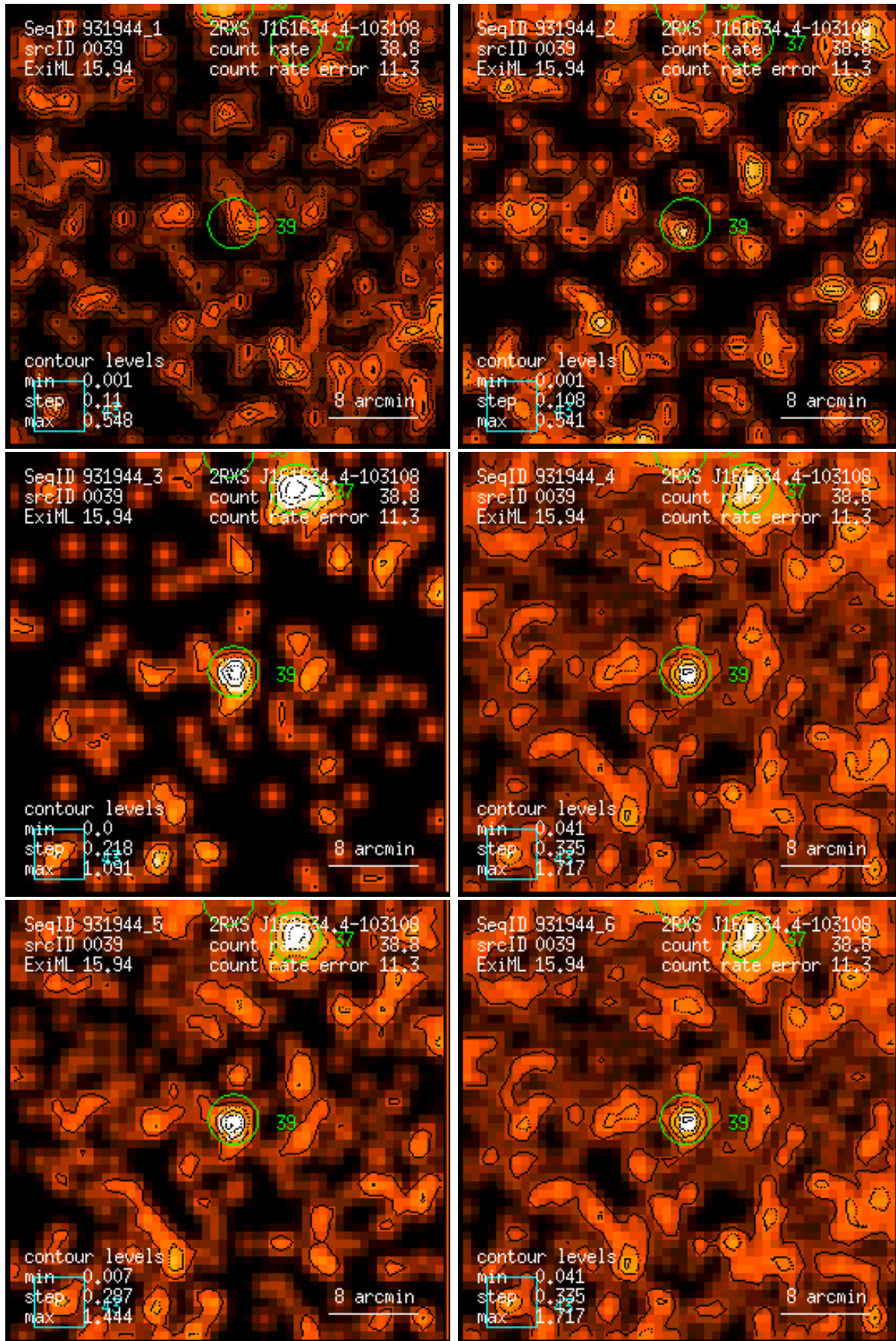
Figure 39: RASS 931944: detection 0039: band rate images, Gaussian filter: (1) PSPC channels 11 – 41, (2) 52 – 90, (3) 91 – 201, (4) 11 – 235, (5) 52 – 201, (6) 11 – 201. Broad band rates in counts/ks. Band rate contour levels in counts/ks/arcmin 2 .
