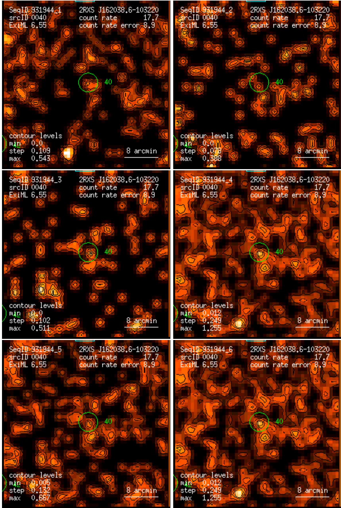
Figure 40: RASS 931944: detection 0040: band rate images, Gaussian filter: (1) PSPC channels 11 – 41, (2) 52 – 90, (3) 91 – 201, (4) 11 – 235, (5) 52 – 201, (6) 11 – 201. Broad band rates in counts/ks. Band rate contour levels in counts/ks/arcmin 2 .
