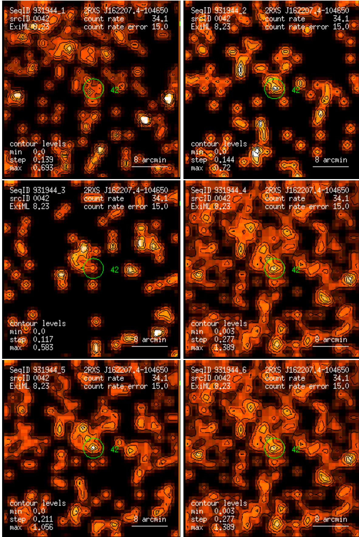
Figure 42: RASS 931944: detection 0042: band rate images, Gaussian filter: (1) PSPC channels 11 – 41, (2) 52 – 90, (3) 91 – 201, (4) 11 – 235, (5) 52 – 201, (6) 11 – 201. Broad band rates in counts/ks. Band rate contour levels in counts/ks/arcmin 2 .
