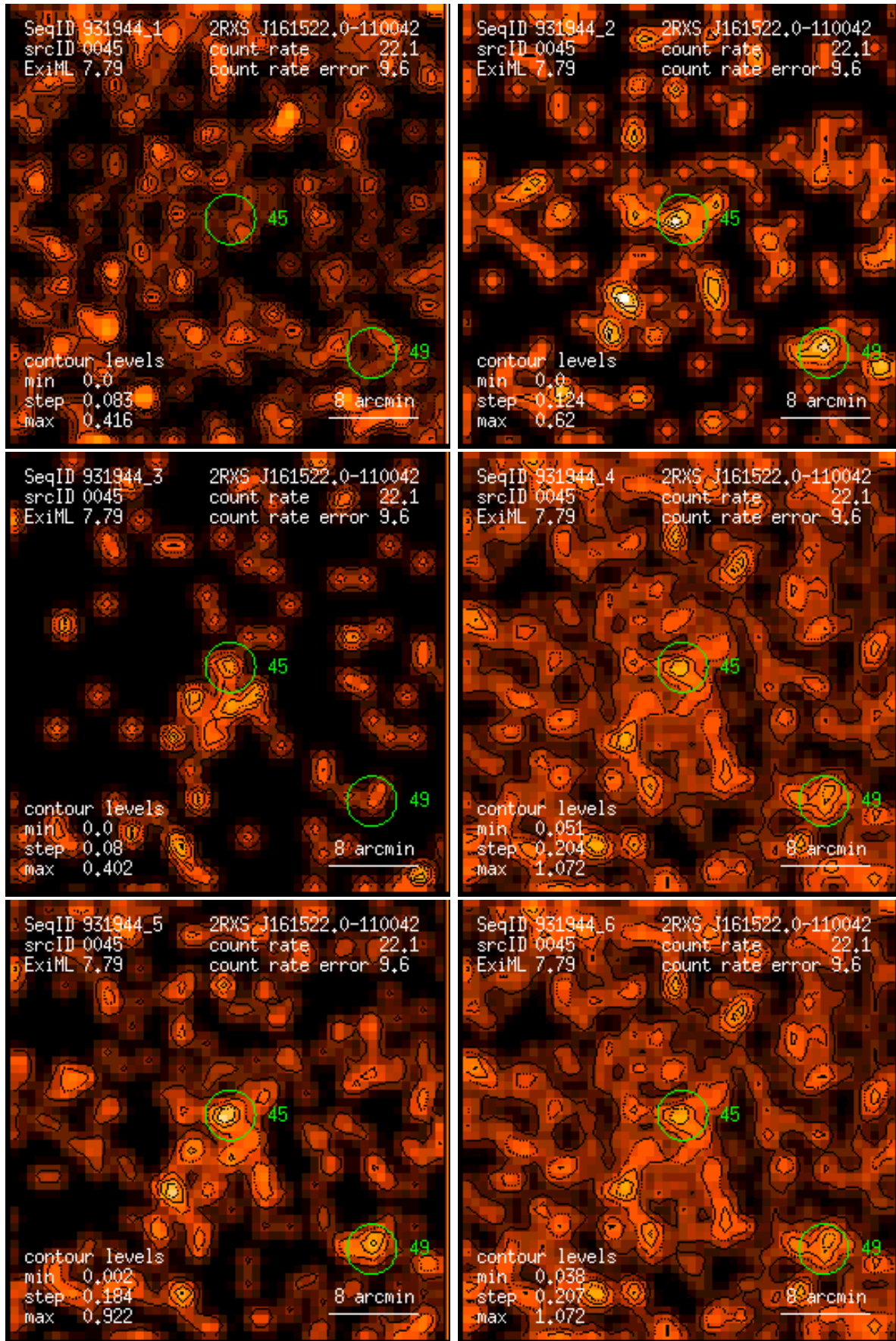
Figure 45: RASS 931944: detection 0045: band rate images, Gaussian filter: (1) PSPC channels 11 – 41, (2) 52 – 90, (3) 91 – 201, (4) 11 – 235, (5) 52 – 201, (6) 11 – 201. Broad band rates in counts/ks. Band rate contour levels in counts/ks/arcmin 2 .
