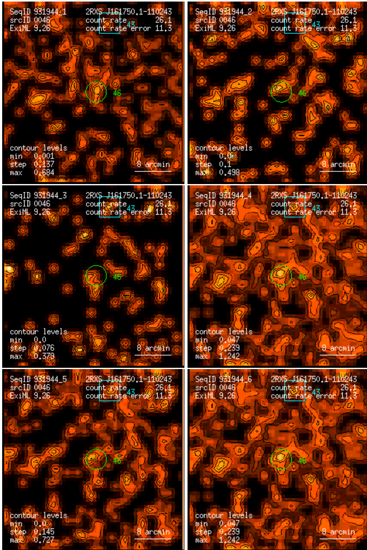
Figure 46: RASS 931944: detection 0046: band rate images, Gaussian filter: (1) PSPC channels 11 – 41, (2) 52 – 90, (3) 91 – 201, (4) 11 – 235, (5) 52 – 201, (6) 11 – 201. Broad band rates in counts/ks. Band rate contour levels in counts/ks/arcmin 2 .
