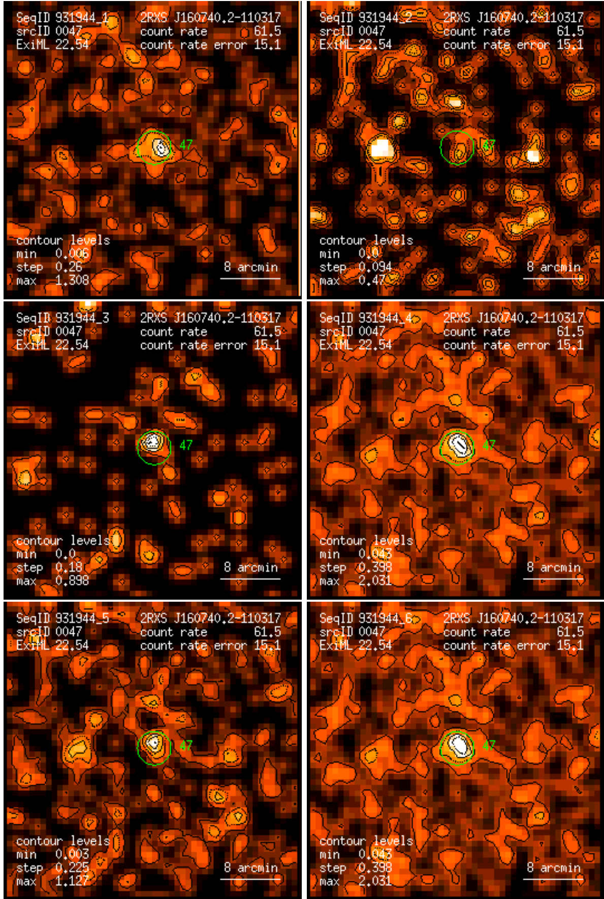
Figure 47: RASS 931944: detection 0047: band rate images, Gaussian filter: (1) PSPC channels 11 – 41, (2) 52 – 90, (3) 91 – 201, (4) 11 – 235, (5) 52 – 201, (6) 11 – 201. Broad band rates in counts/ks. Band rate contour levels in counts/ks/arcmin 2 .
