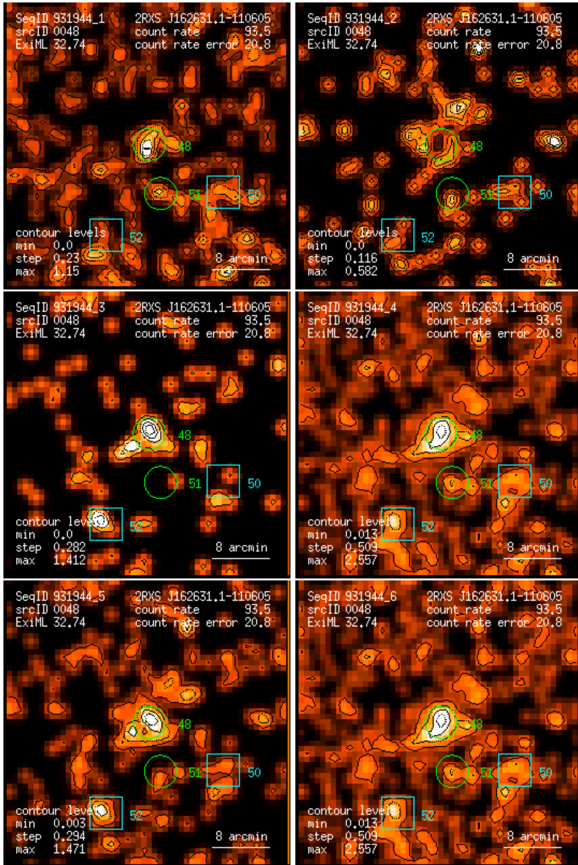
Figure 48: RASS 931944: detection 0048: band rate images, Gaussian filter: (1) PSPC channels 11 – 41, (2) 52 – 90, (3) 91 – 201, (4) 11 – 235, (5) 52 – 201, (6) 11 – 201. Broad band rates in counts/ks. Band rate contour levels in counts/ks/arcmin 2 .
