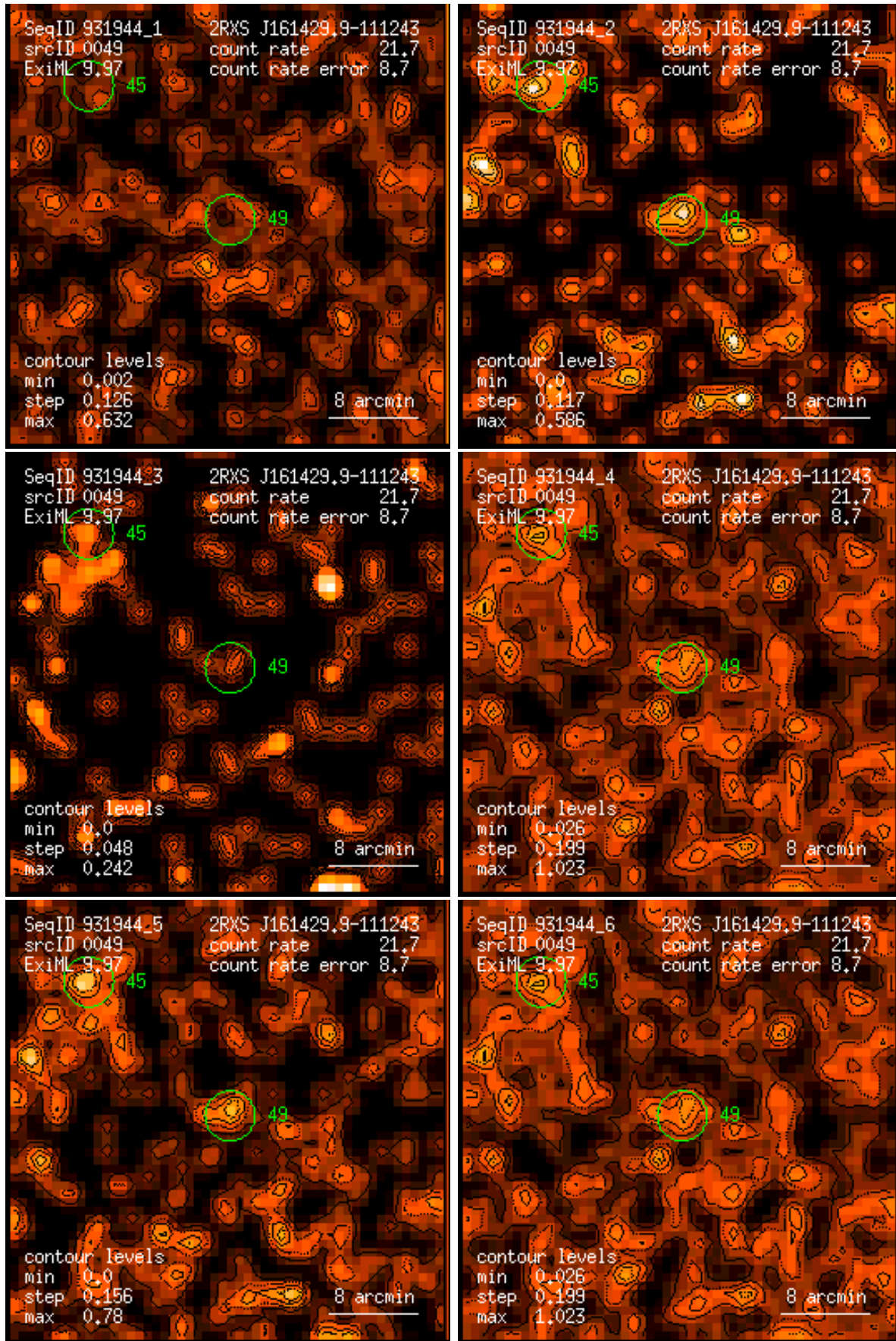
Figure 49: RASS 931944: detection 0049: band rate images, Gaussian filter: (1) PSPC channels 11 – 41, (2) 52 – 90, (3) 91 – 201, (4) 11 – 235, (5) 52 – 201, (6) 11 – 201. Broad band rates in counts/ks. Band rate contour levels in counts/ks/arcmin 2 .
