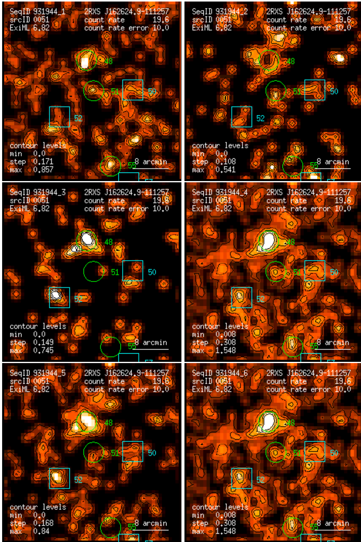
Figure 51: RASS 931944: detection 0051: band rate images, Gaussian filter: (1) PSPC channels 11 – 41, (2) 52 – 90, (3) 91 – 201, (4) 11 – 235, (5) 52 – 201, (6) 11 – 201. Broad band rates in counts/ks. Band rate contour levels in counts/ks/arcmin 2 .
