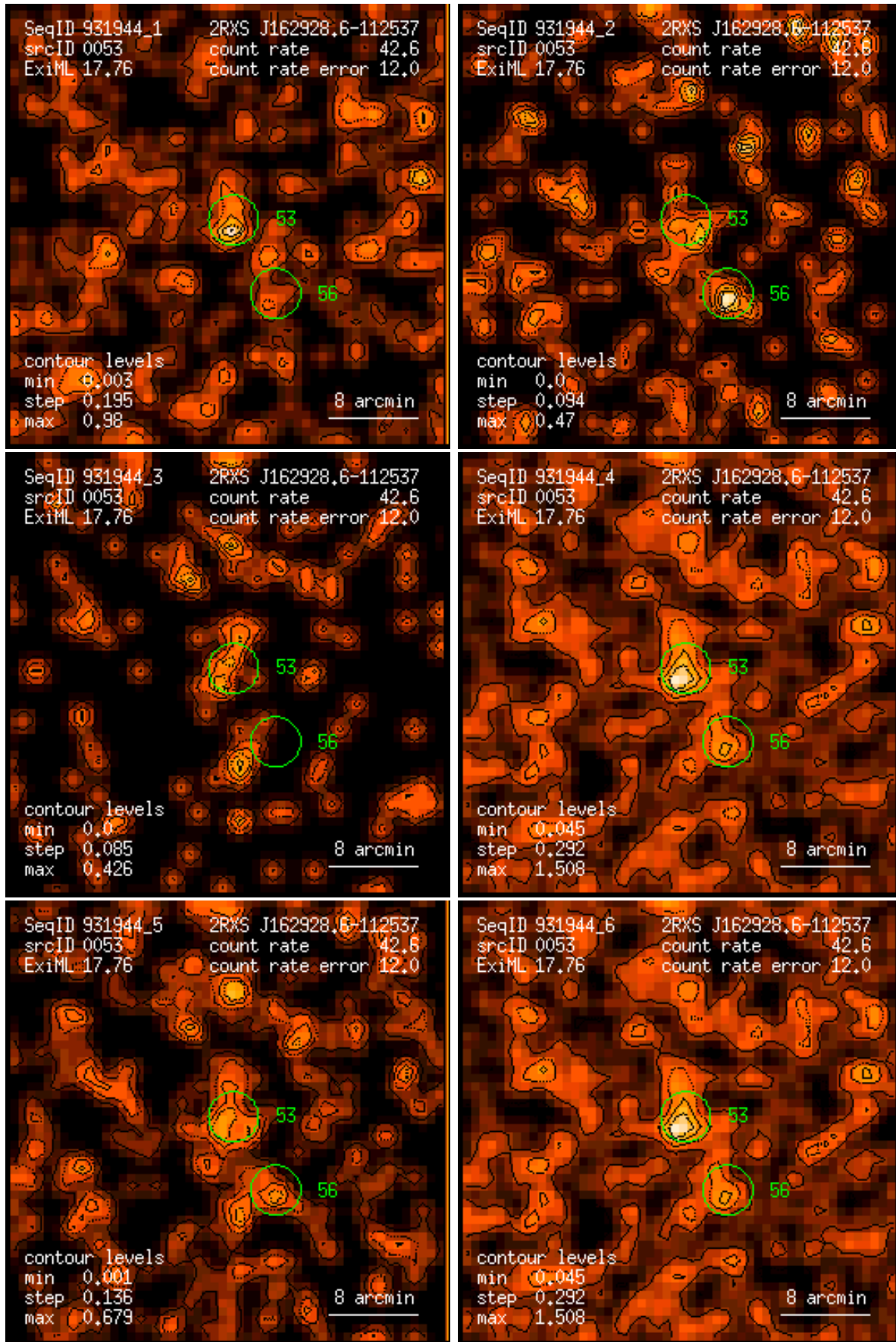
Figure 53: RASS 931944: detection 0053: band rate images, Gaussian filter: (1) PSPC channels 11 – 41, (2) 52 – 90, (3) 91 – 201, (4) 11 – 235, (5) 52 – 201, (6) 11 – 201. Broad band rates in counts/ks. Band rate contour levels in counts/ks/arcmin 2 .
