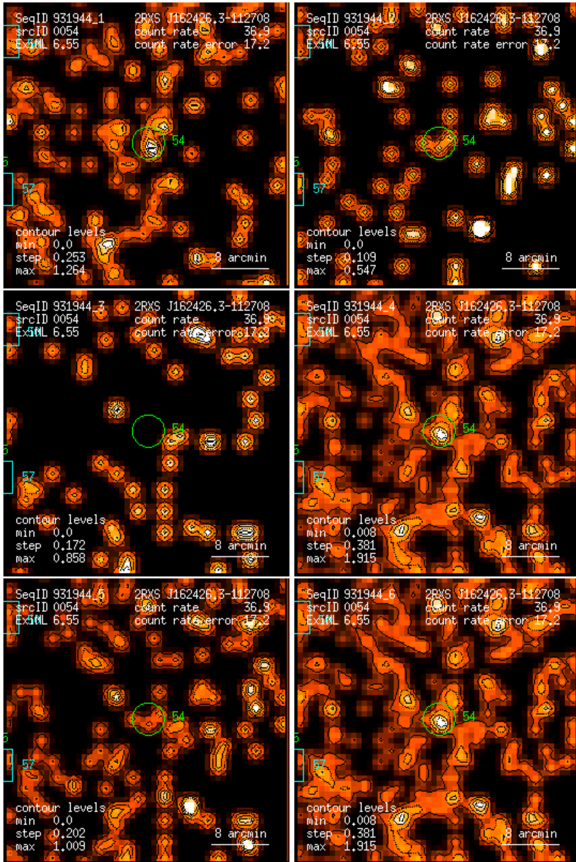
Figure 54: RASS 931944: detection 0054: band rate images, Gaussian filter: (1) PSPC channels 11 – 41, (2) 52 – 90, (3) 91 – 201, (4) 11 – 235, (5) 52 – 201, (6) 11 – 201. Broad band rates in counts/ks. Band rate contour levels in counts/ks/arcmin 2 .
