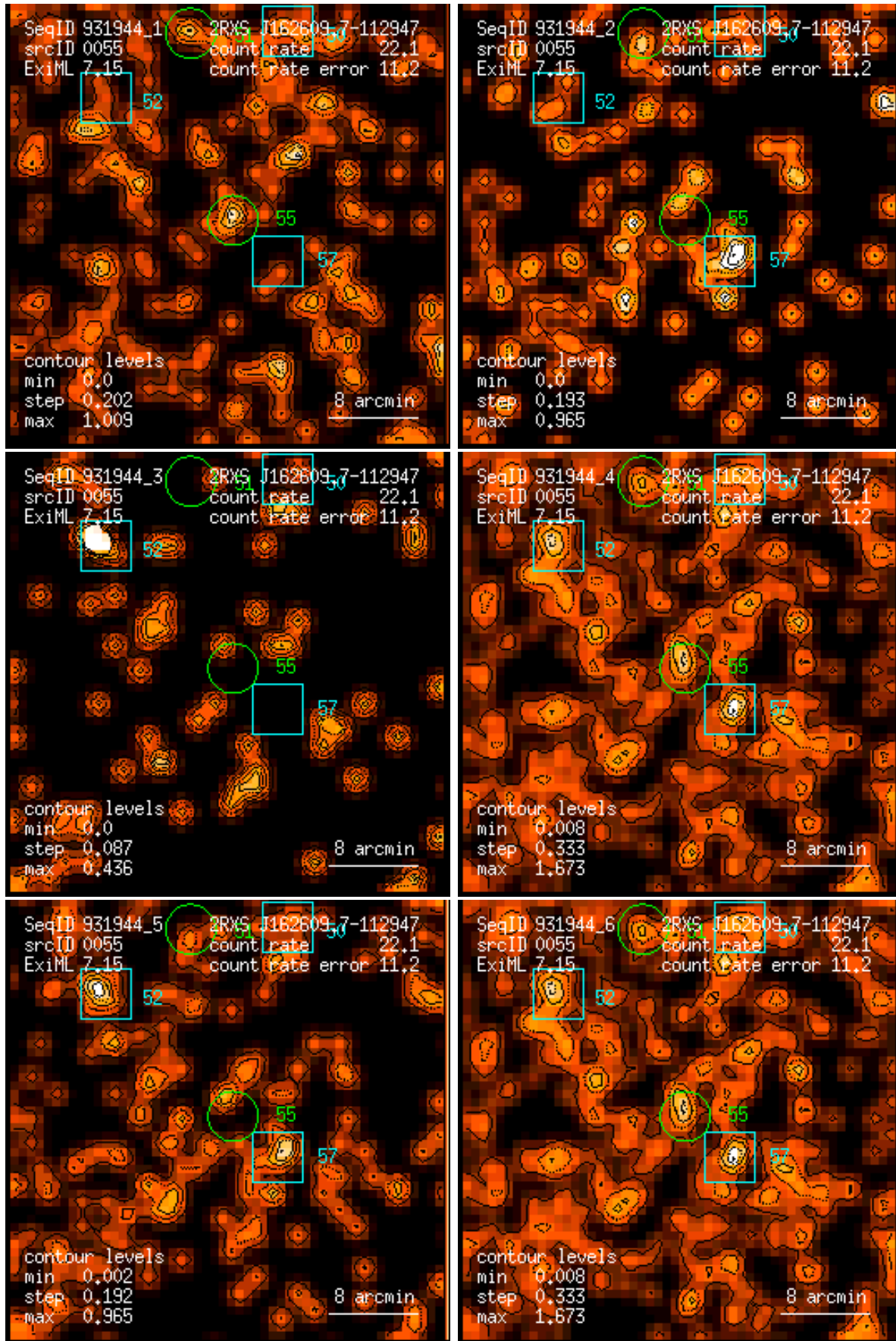
Figure 55: RASS 931944: detection 0055: band rate images, Gaussian filter: (1) PSPC channels 11 – 41, (2) 52 – 90, (3) 91 – 201, (4) 11 – 235, (5) 52 – 201, (6) 11 – 201. Broad band rates in counts/ks. Band rate contour levels in counts/ks/arcmin 2 .
